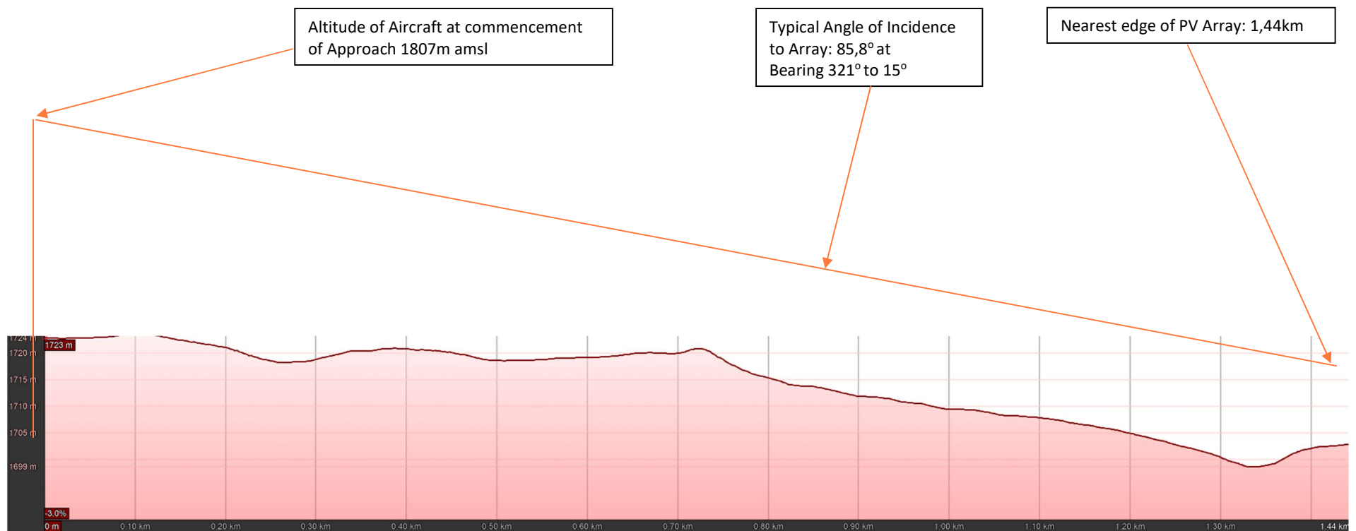
Figure 16: Aircraft Approaching RWY 32 (E-W): Typical Geometry to Solar Array
