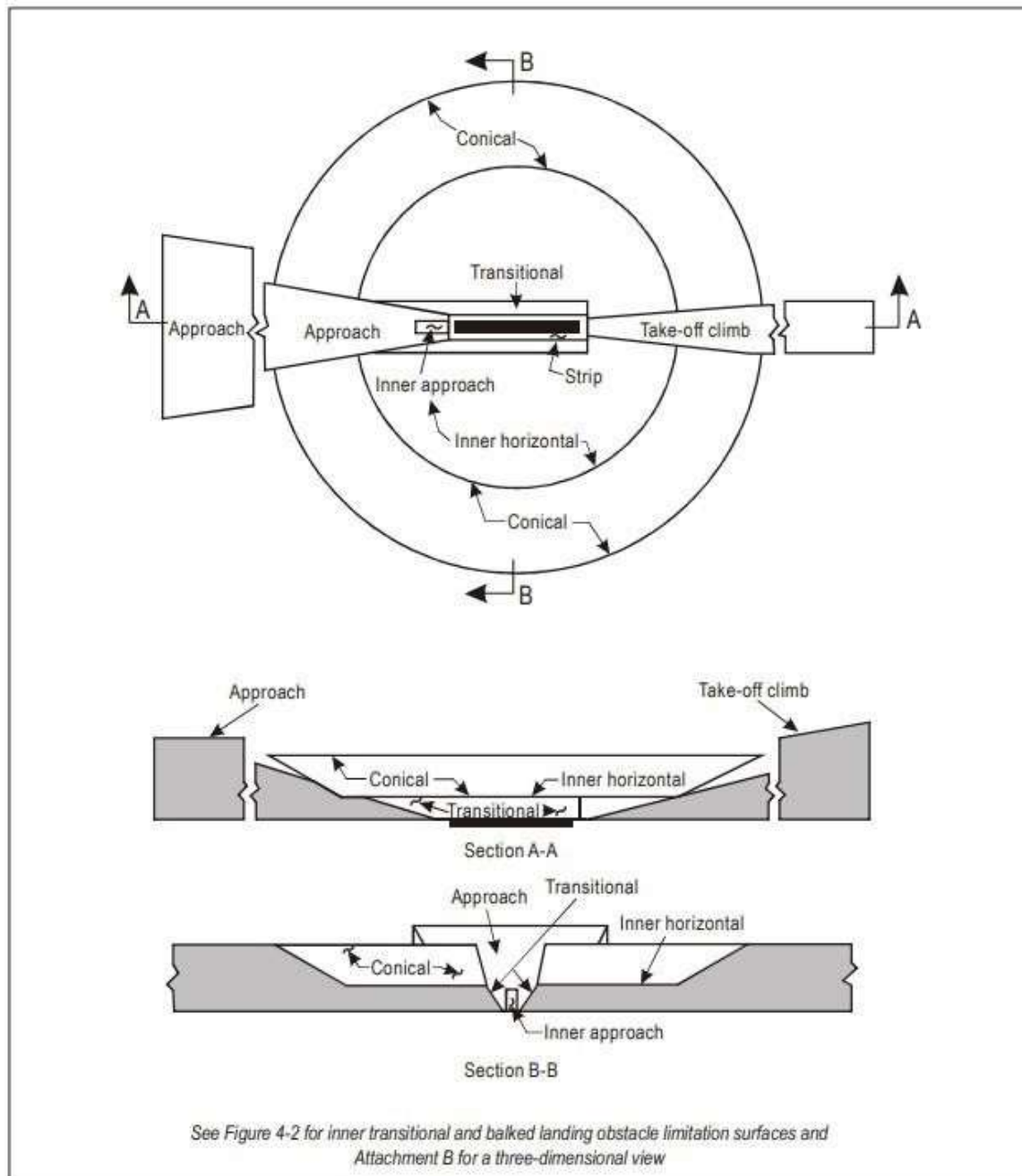
Figure 3: ICAO Obstacle Limitation Surfaces
