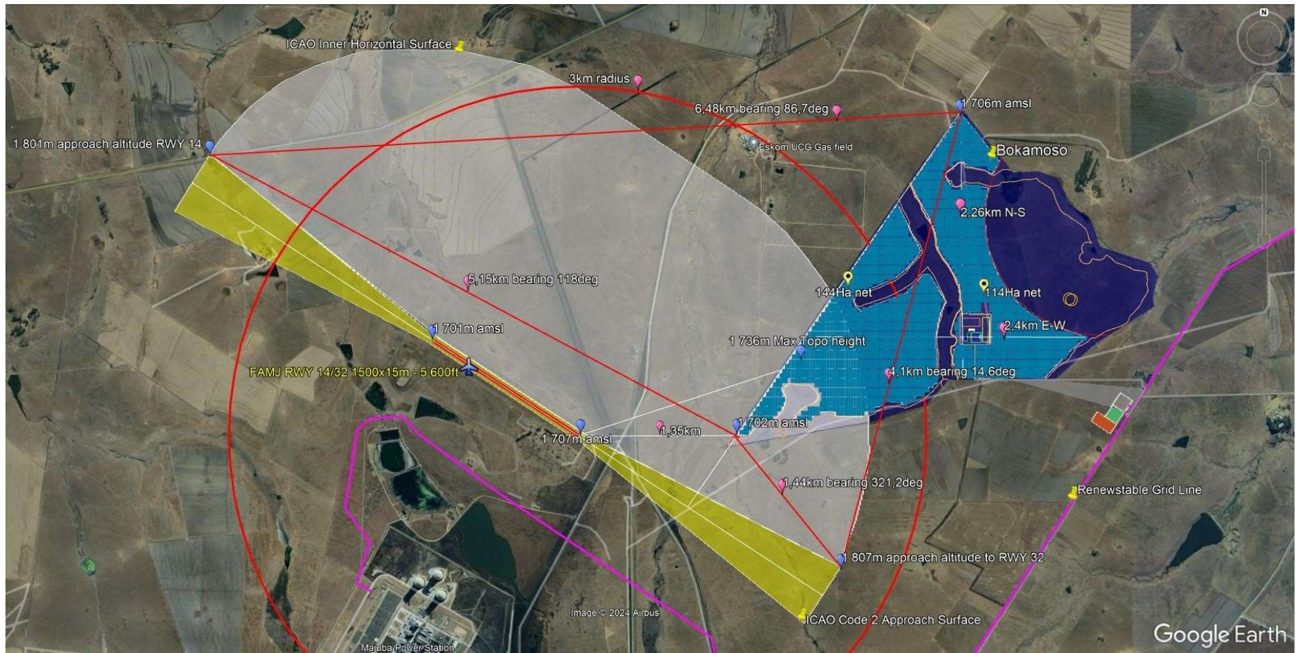
Figure 14: Approach Surfaces to FAMJ RWY14/32 with key distances & bearings to Bokamoso Solar Array
